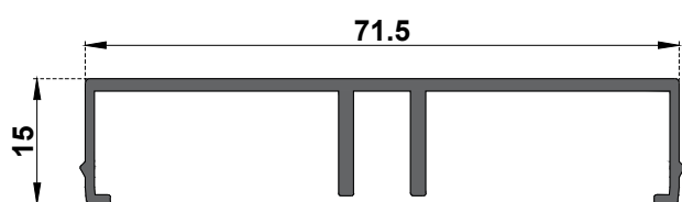
93604 kg/m 0.505
