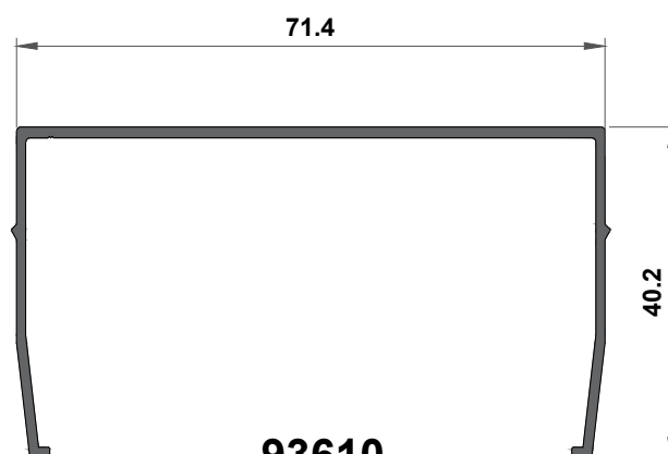
93610 kg/m 0.502
