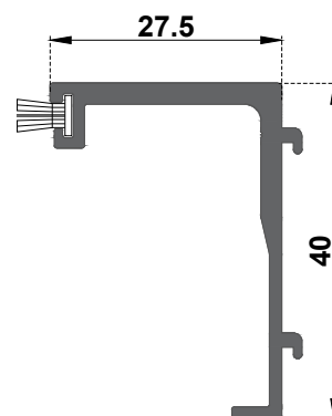
93606 kg/m 0.452
