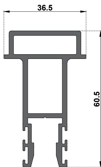
93601 kg/m 1.159
