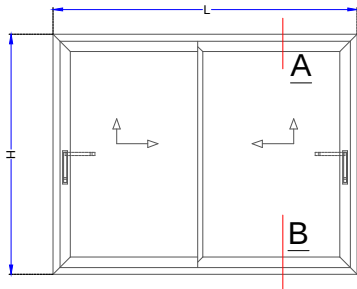
Kanati qendror minimal (Minimal central sash)
